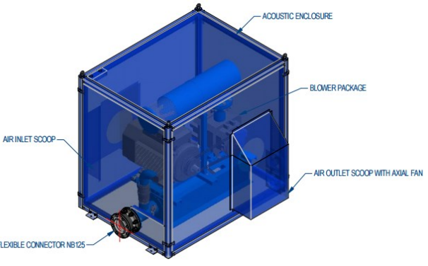
Roots Blower Packages with Acoustic Enclosure
