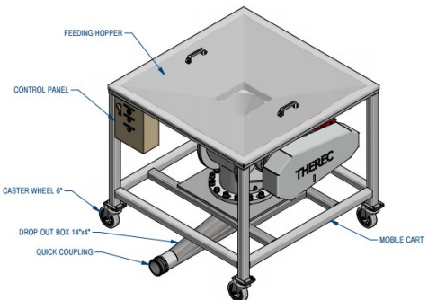
Mobiled High-Pressure Air-Lock Rotary Valves
